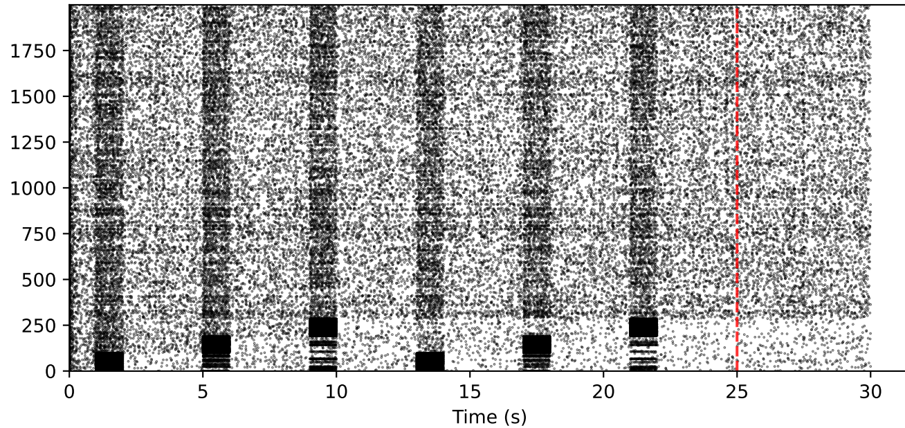
With iSTDP
