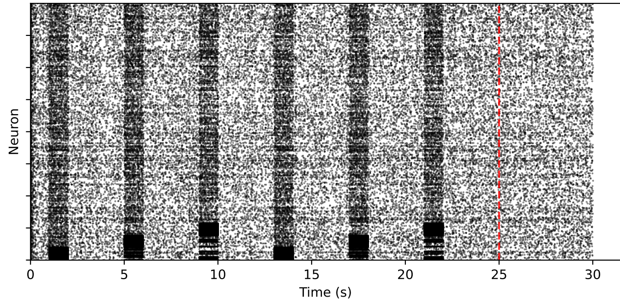
Without iSTDP
